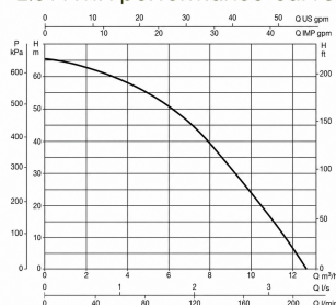
E.SYTWIN performance curve
