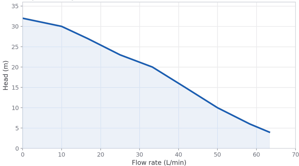
Esybox POP performance curve
