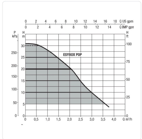
DAB Esybox Pop — head (H) vs flow (Q). Indicative curve; actual performance varies with installation conditions.
