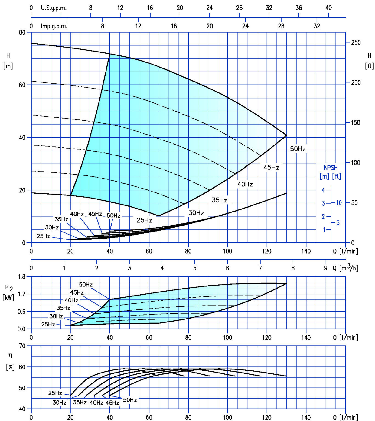
EVMS(.)-K5 8/2.2
