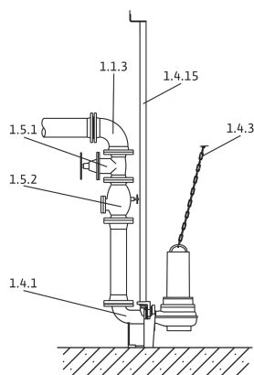
Installation drawing
