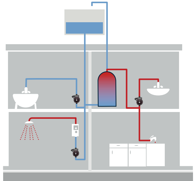
Illustration does not show non-return valves.
