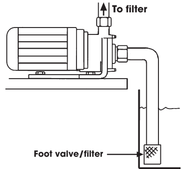
Fig 2:-Suction Lift
