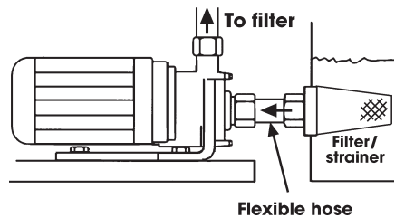
FIG 3:- Gravity Feed
