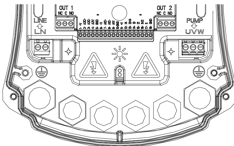
Figure 1: Electrical connections
