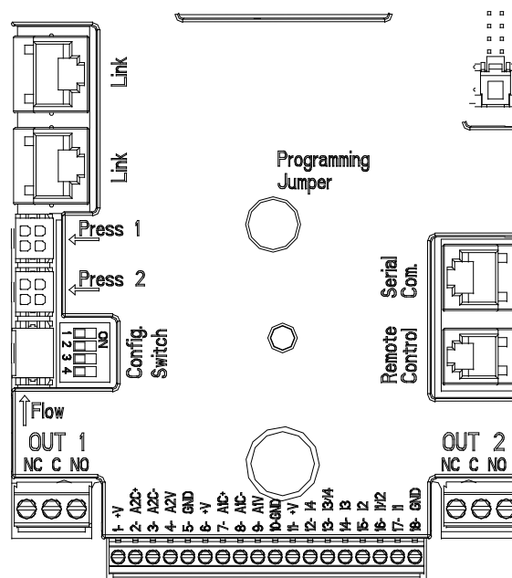
Figure 3: Connections
