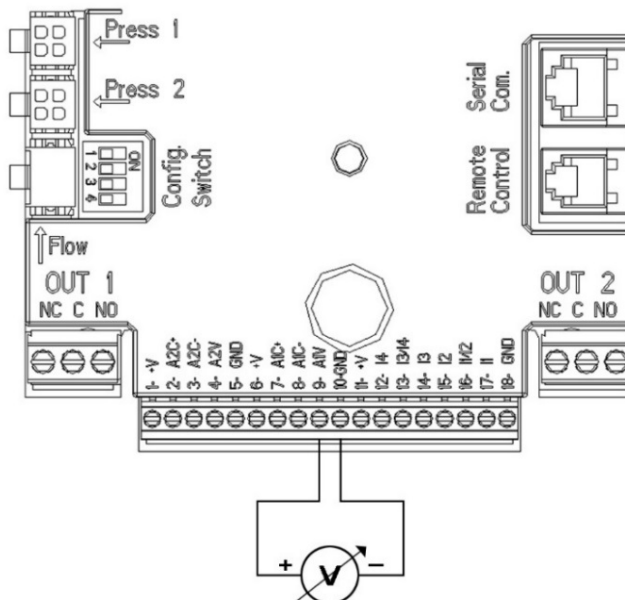
Figure 6: Example of Connection of Analogue Input
